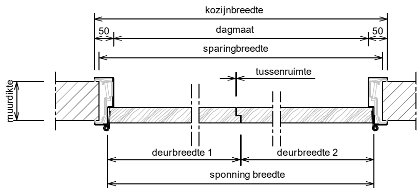
Horizontale doorsnede (loop-stand)
