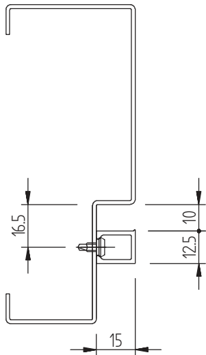
aluminium 13x15
