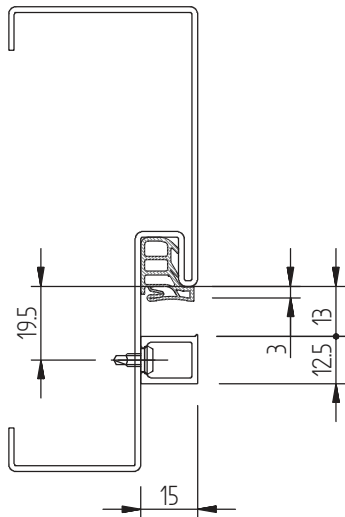
aluminium 13x15
